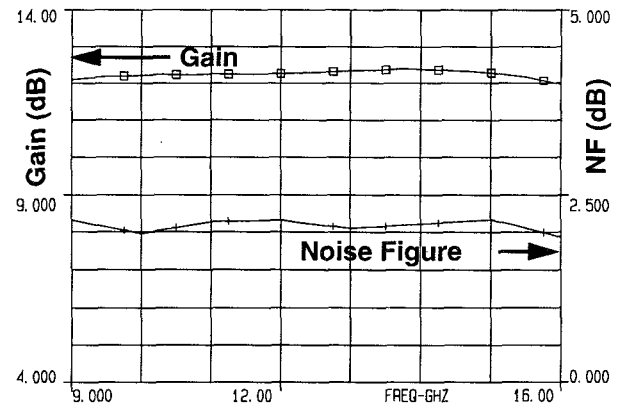
Fig. 2 On-wafer measurements of S-parameters and Noise Figure.
